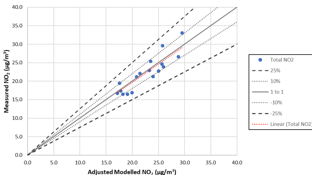
Figure 1-2: Adjusted model verification (annual mean NO 2 ; µg/m 3 )
